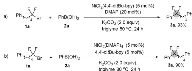
Scheme 2. The role of DMAP.
